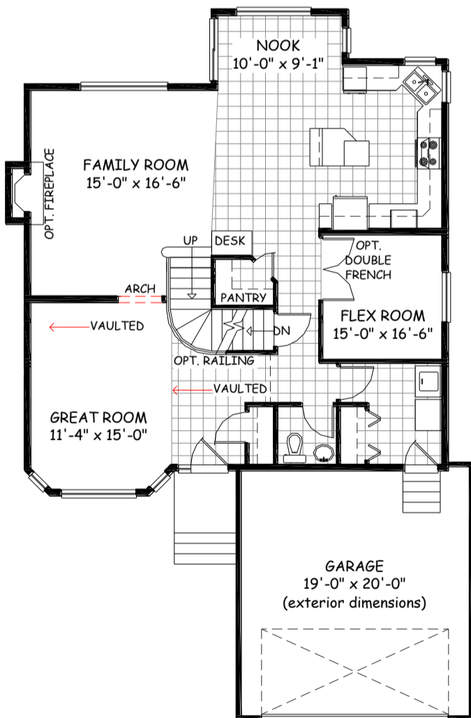
Main Floor 1164 sq. ft.
